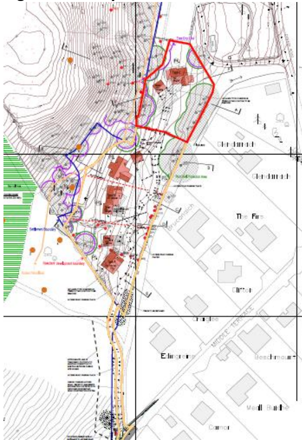
Figure 2 Site Layout
