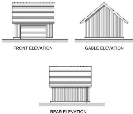
Figure 4 – Proposed Garage
